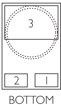
Figure 9a. LUXEON Rebel Color Line pad configuration.
